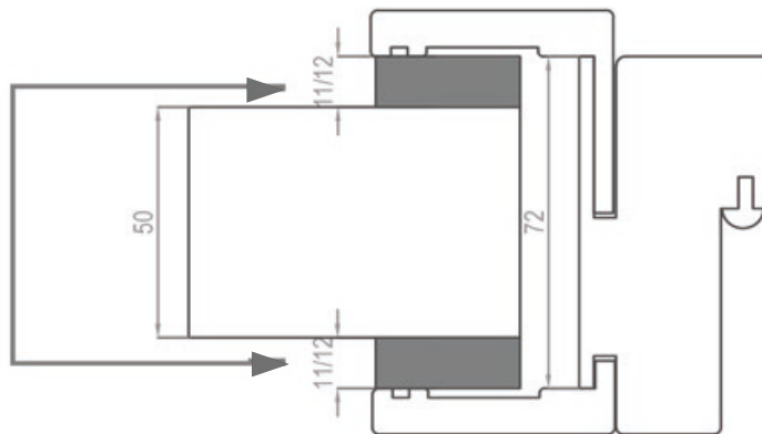
CADRE 72MM > CLOISON 50MM
