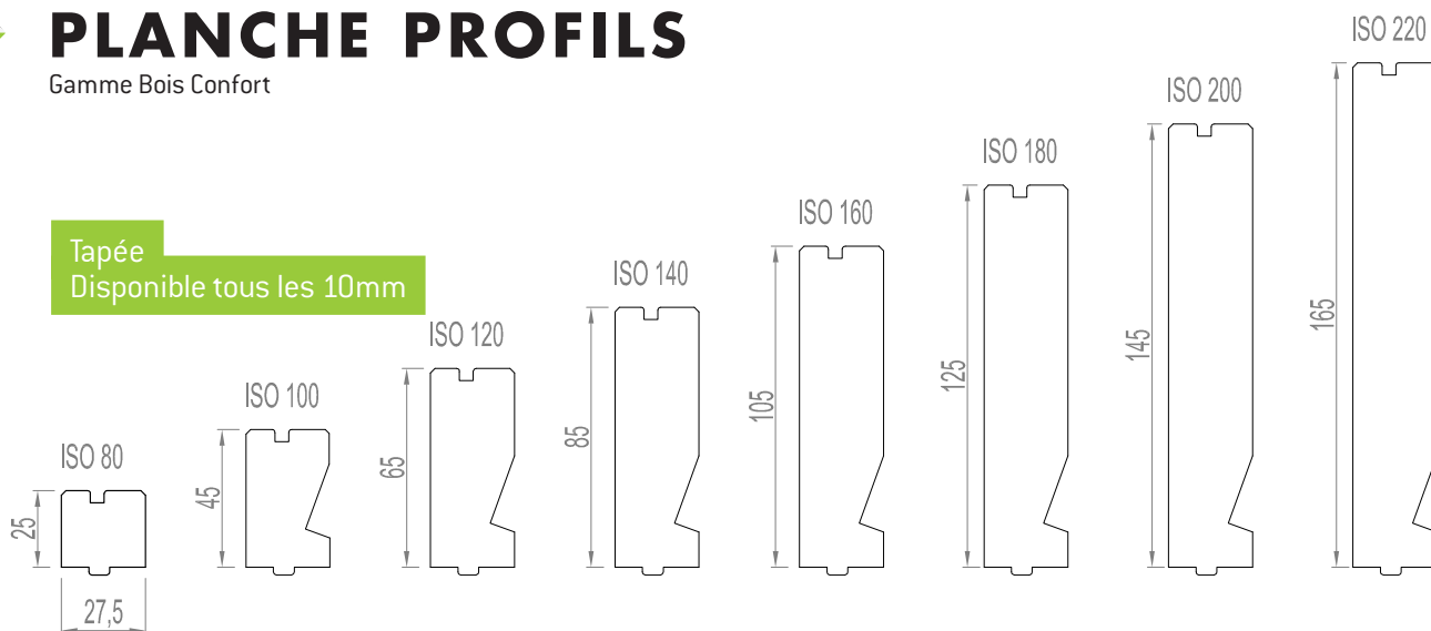
Dormant standard
