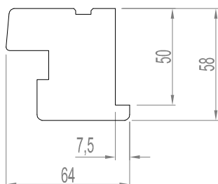
Dormant standard
